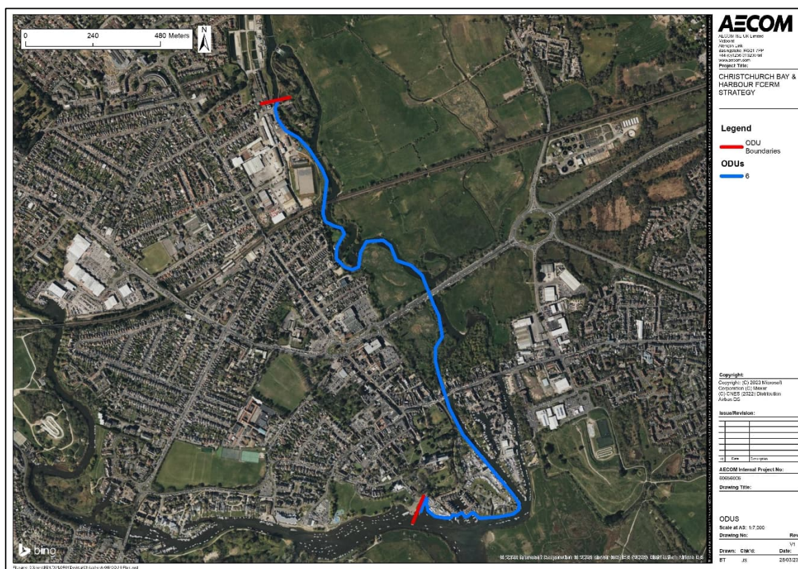
Figure 11.1 ODU 6
