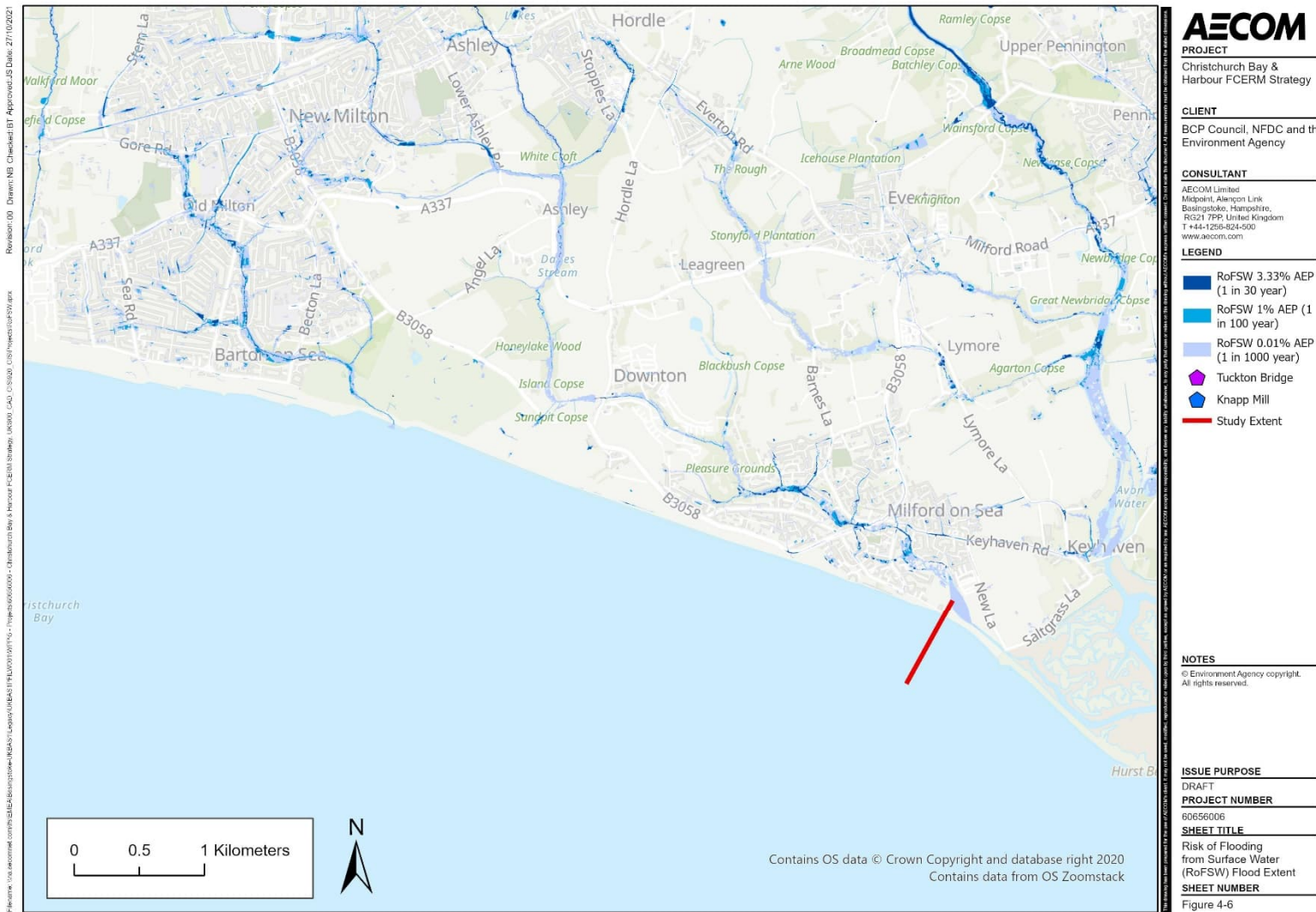
Figure 4-6: Surface Water Flood Risk from Barton-on-Sea to Milford-on-Sea
